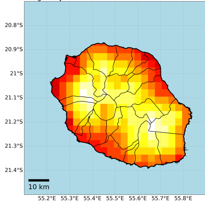
Average daily maximum Heat Index - 2071-2100 - SSP2-4.5
