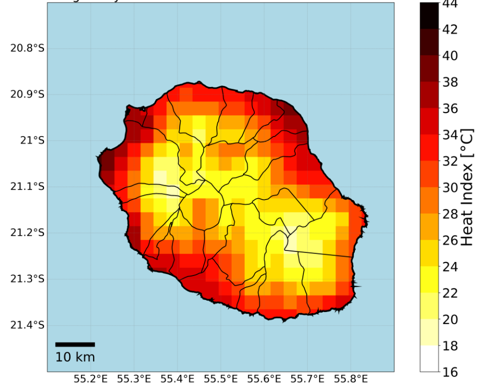
Average daily maximum Heat Index - 2071-2100 - SSP5-8.5
